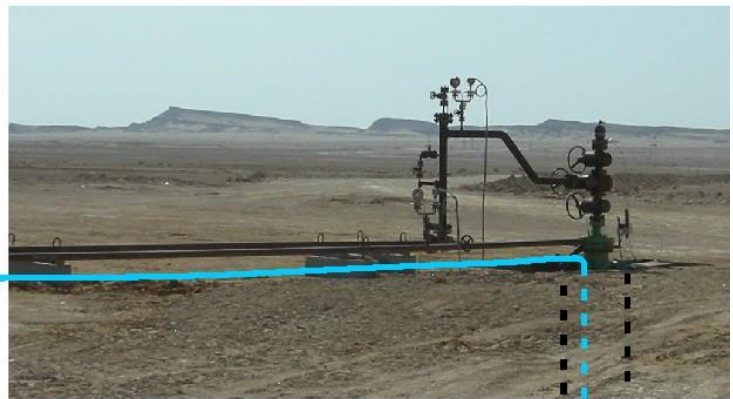
Downhole optical cable
