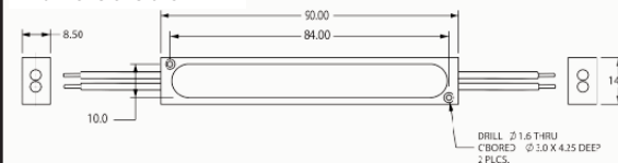
Figure 3: Dimensions of 1x2 or 2x2 Fused Splitter With 3mm Cabled Fibers (Version 2)
